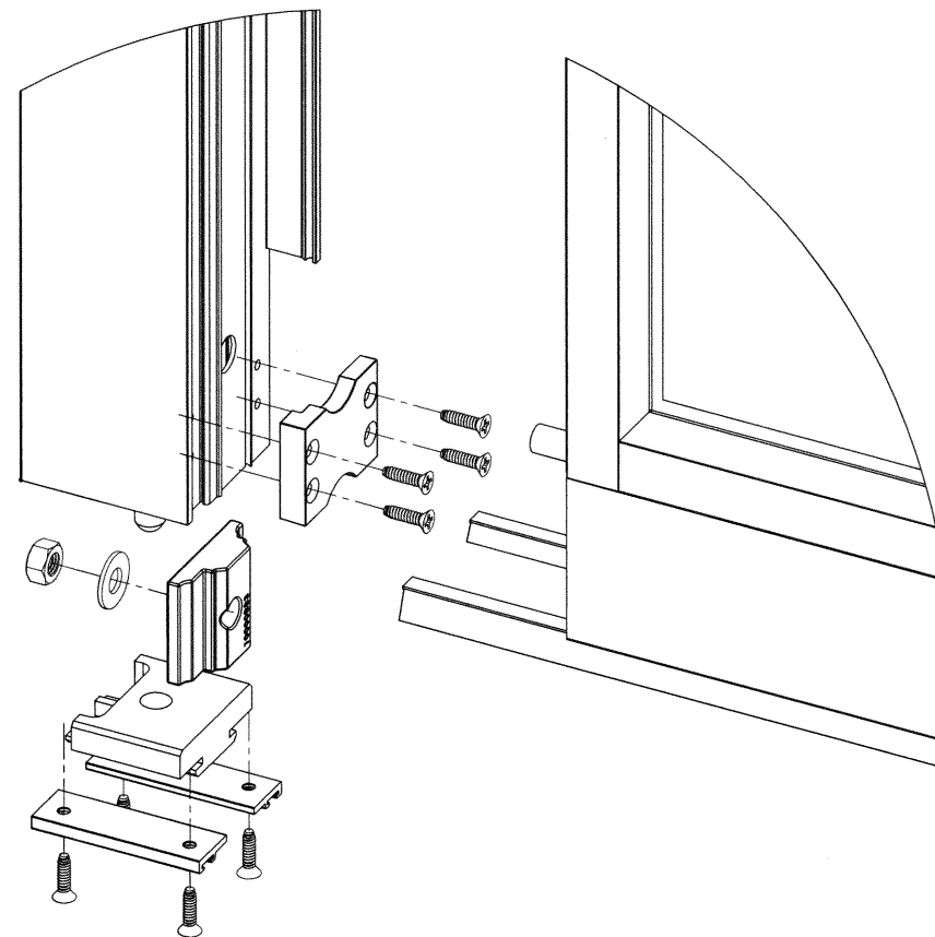
PANEL CORNER
