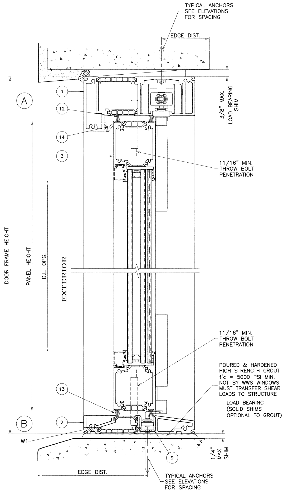
E-3 FRAME OPTION
