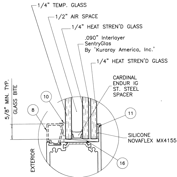
GLAZING DETAIL
